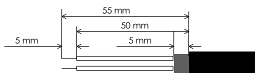
Fig. 2 Cable preparation
