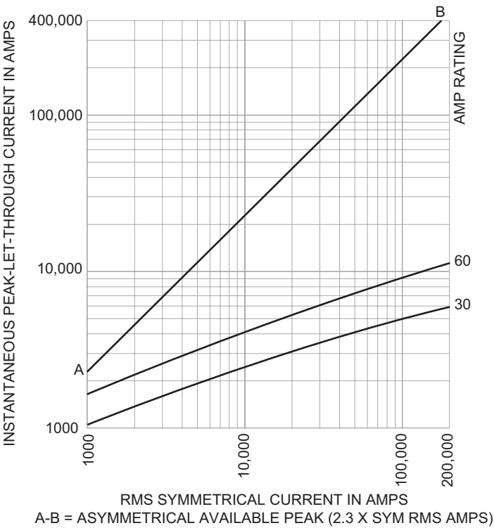
Current-limitation curves — applies only to 600 Vac fuses
