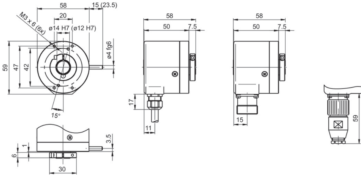
G0M2H - clamping ring on flange
