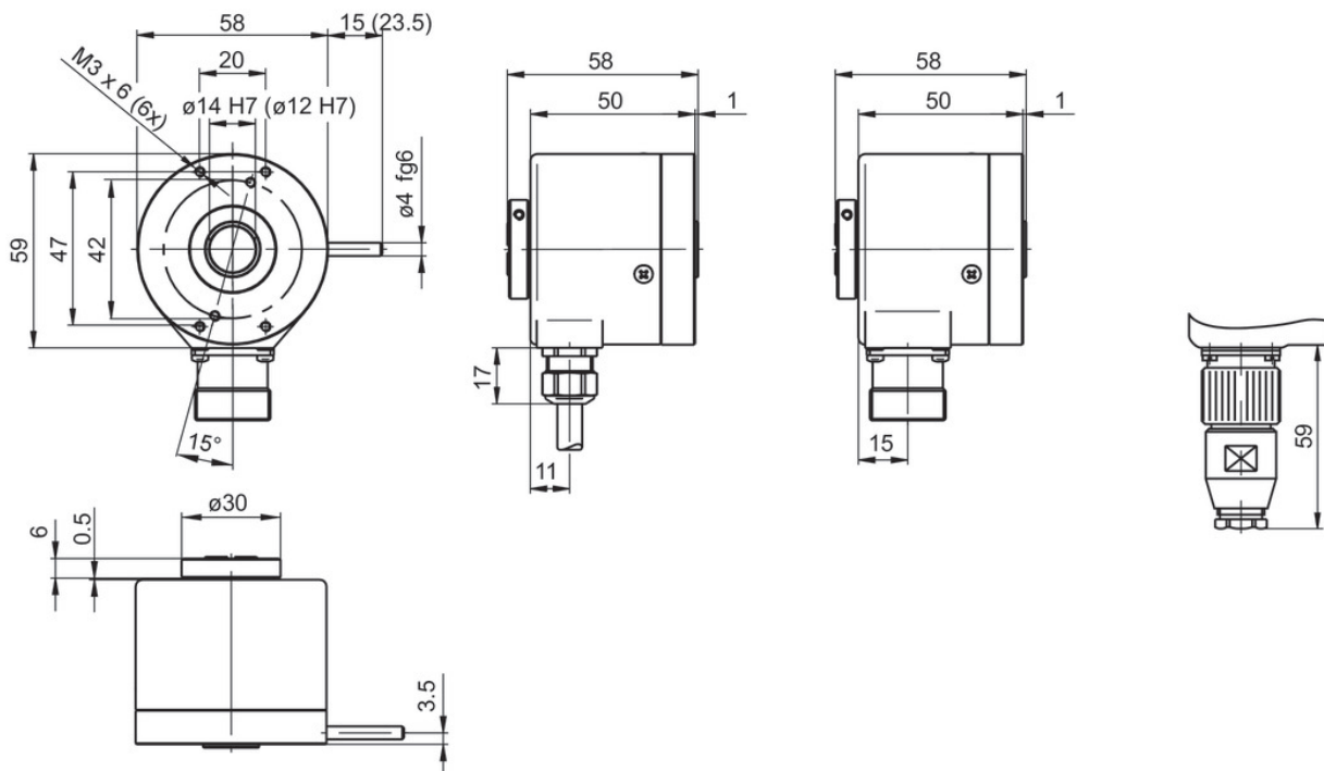
G0M2H - clamping ring on housing
