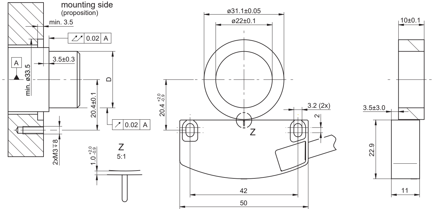
EB260.IR-5N with EBS.R-5N022.B for bonding
