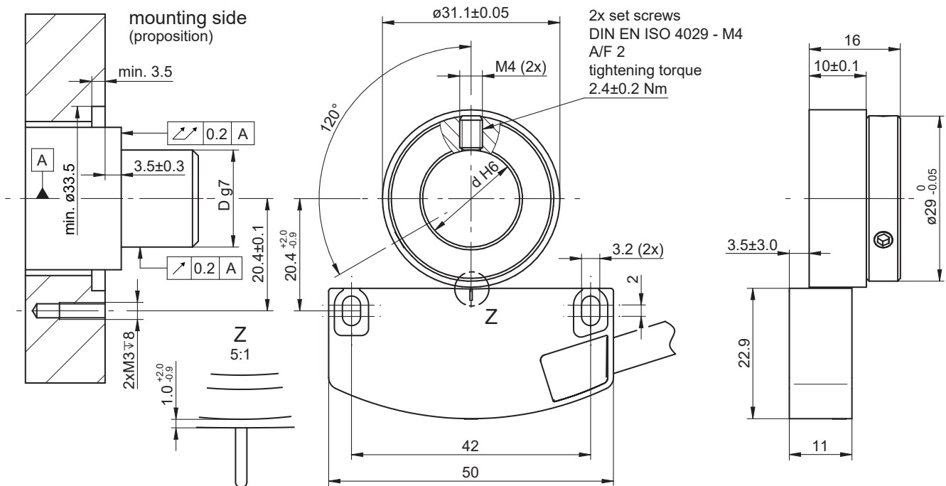
EB260.IR-5N with EBS.R-5N022.S for screw mounting
