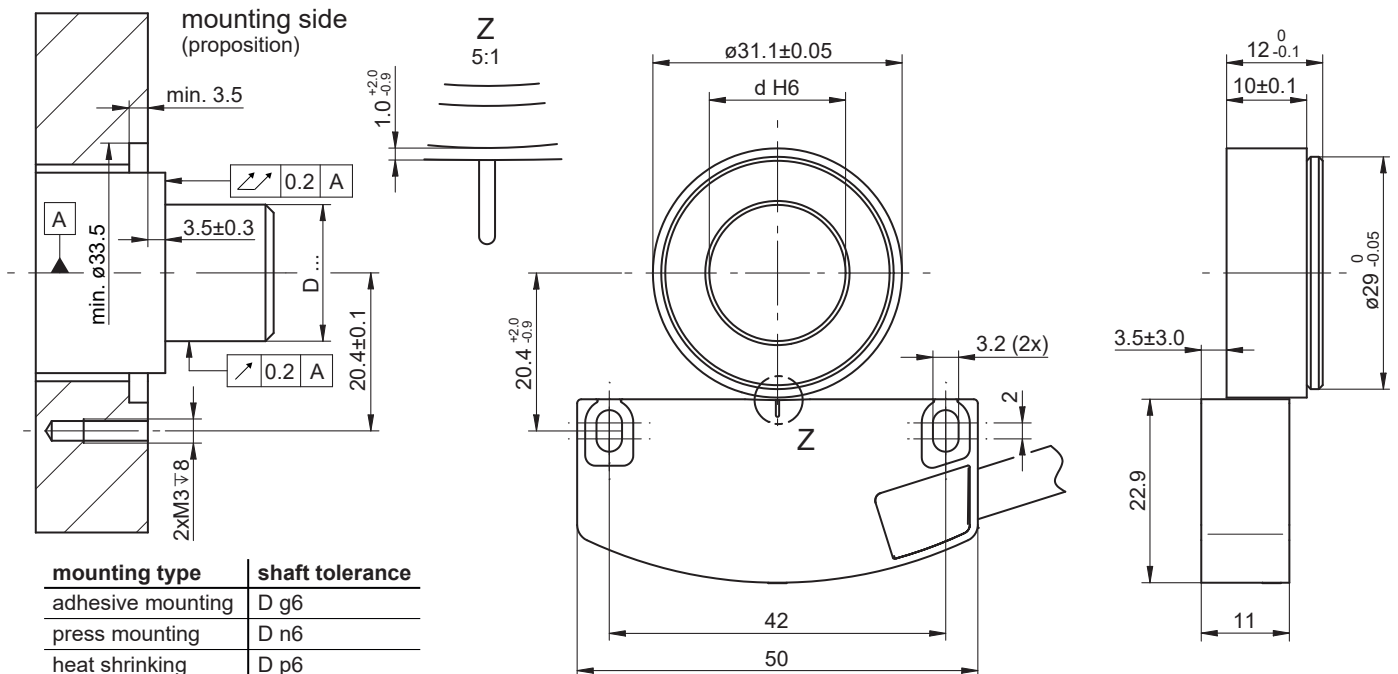
EB260.IR-5N with EBS.R-5N022.U for universal mounting (gluing / pressing / heat shrinking)
