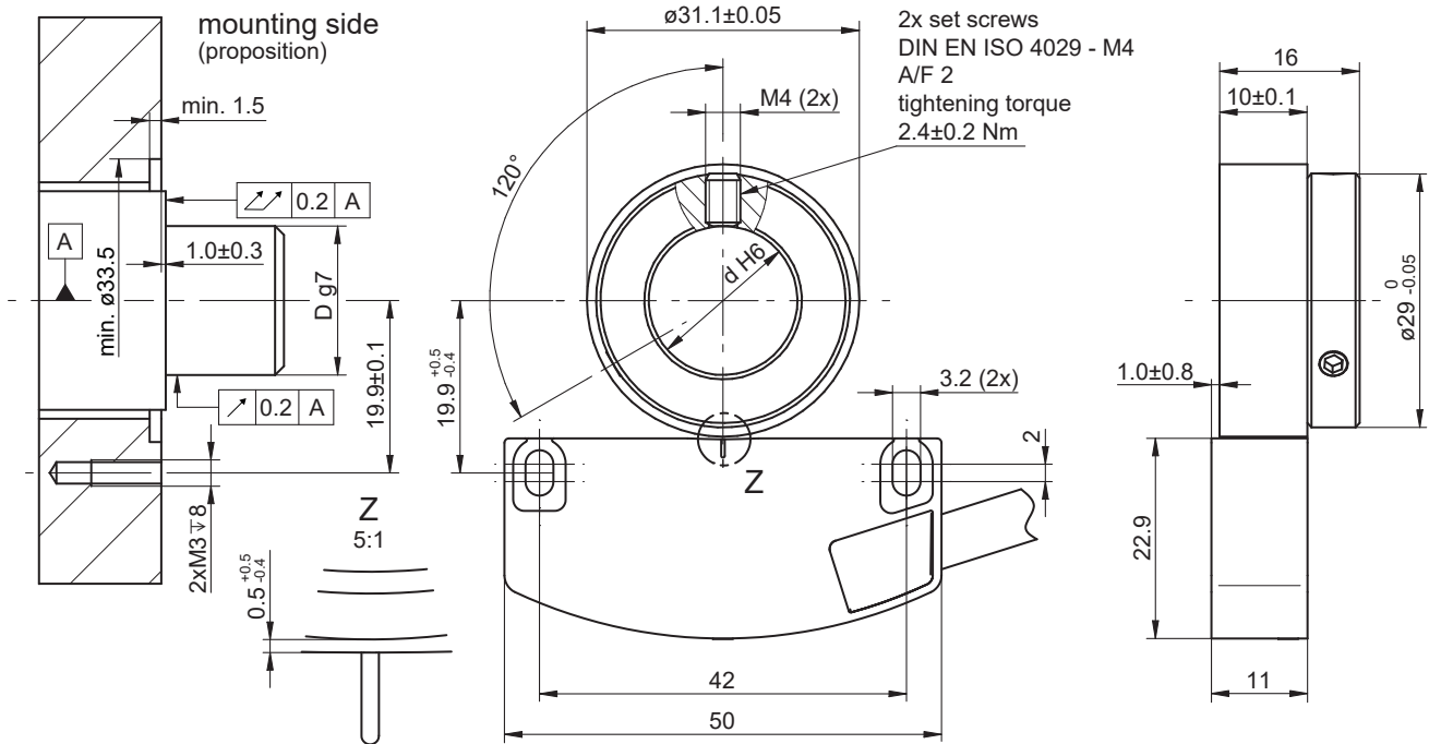
EB260F.IR-2R with EBS.R-2R052.S for screw mounting
