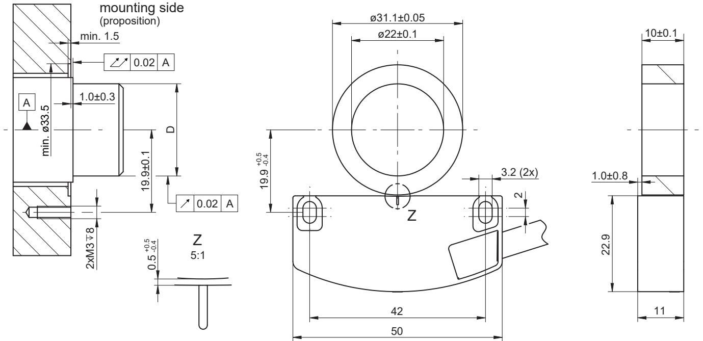
EB260F.IR-2R with EBS.R-2R052.B for bonding
