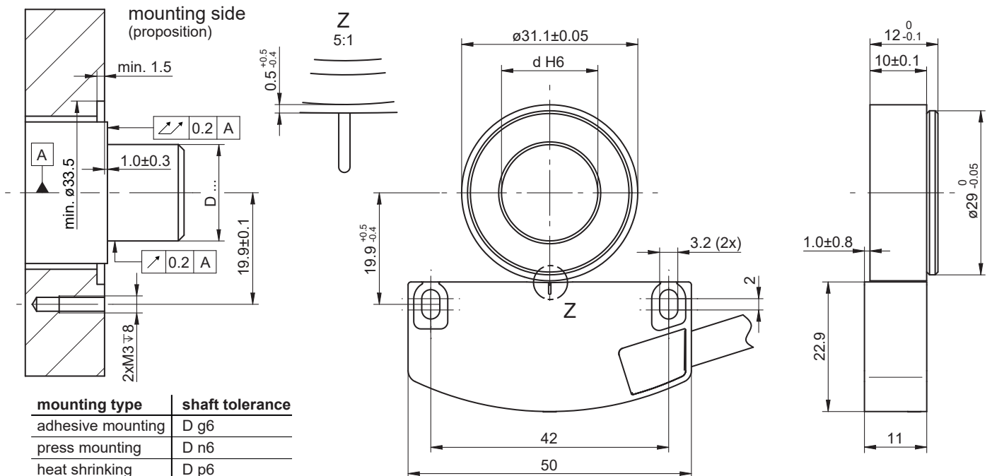
EB260F.IR-2R with EBS.R-2R052.U for universal mounting (gluing / pressing / heat shrinking)
