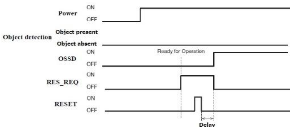
Figure 4-8 Manual restart sequence
