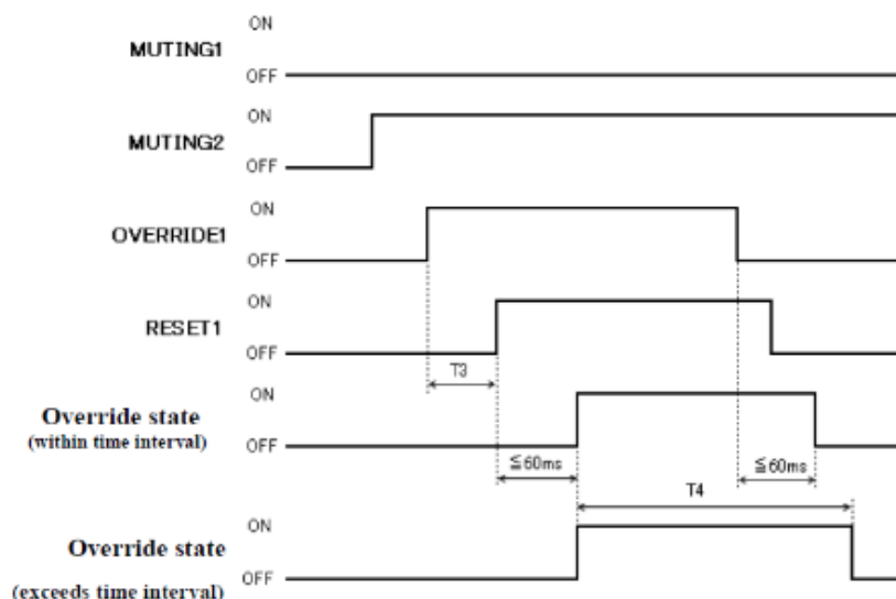
Figure4-12 Override sequence
