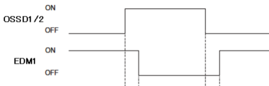
Figure 4-10 EDM timing chart
