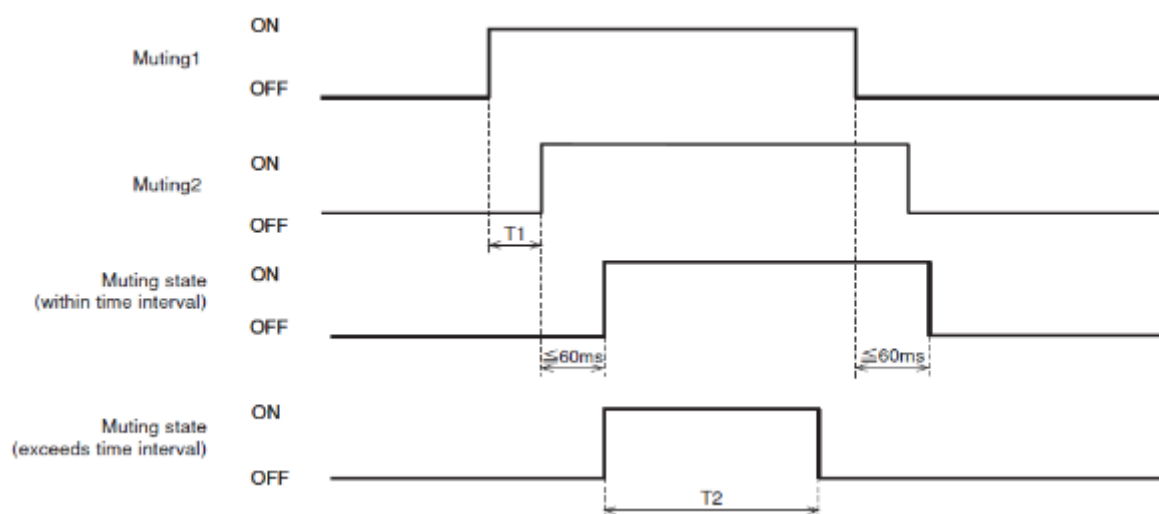
Figure 4-11 Muting sequence
