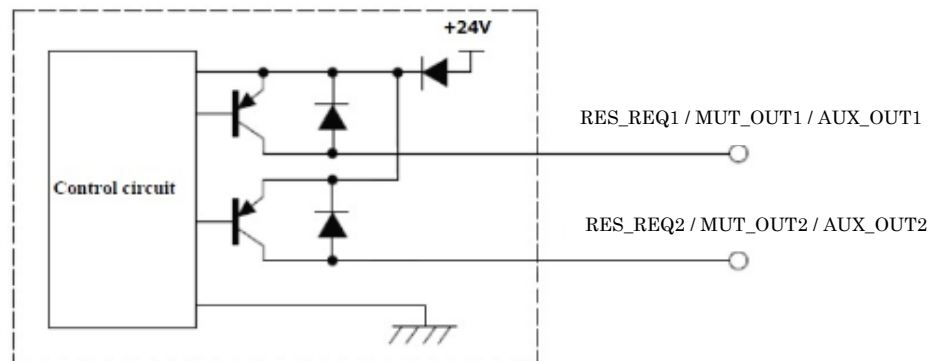
Figure 6-2 Output circuit
