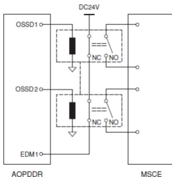
Figure4-9 EDM circuit
