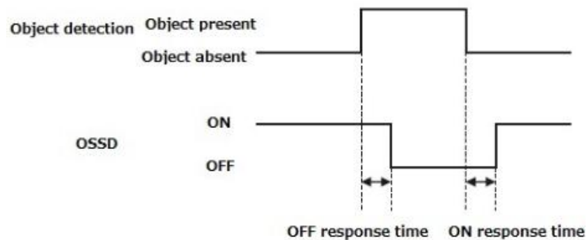
Figure4-6 Timing chart of automatic restart
