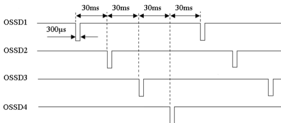
Figure4-5 Timing chart of the OSSD's self-diagnostic function
