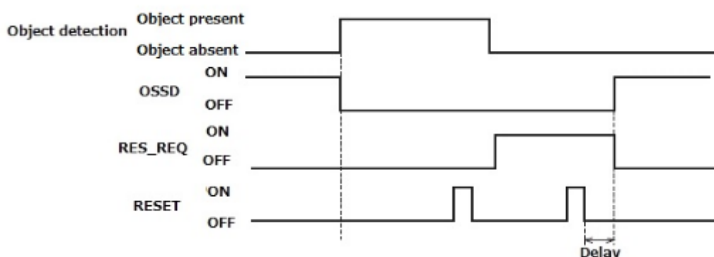
Figure 4-7 Manual restart timing chart
