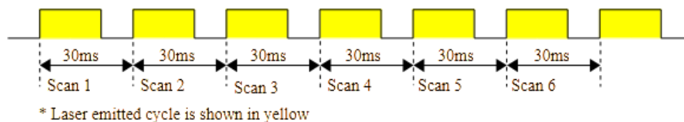
Figure 4-21 Operation of UAM when scan skip count is 0
