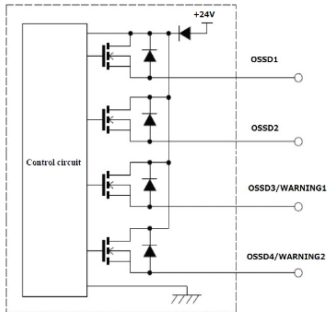
Figure 6-1 OSSD/WARNING Output circuit
