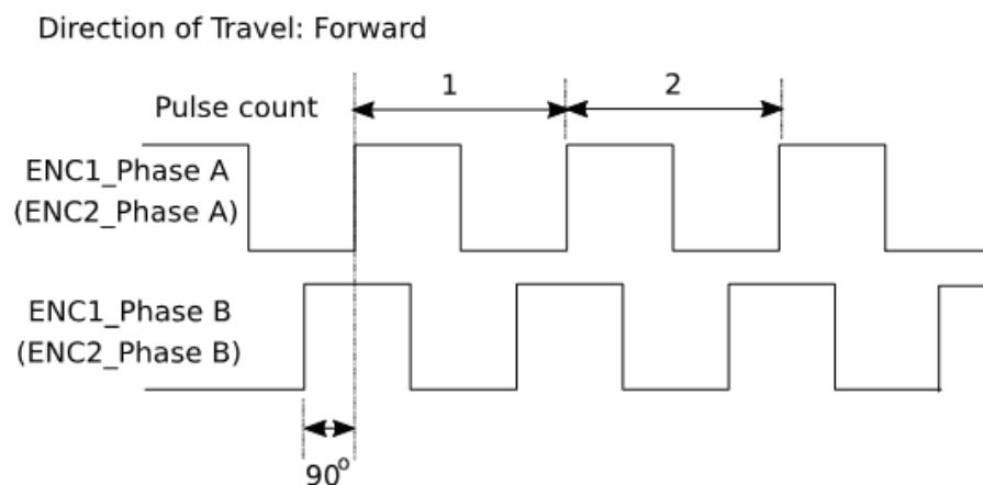
Figure 4-17 Input signal through Incremental encoder
