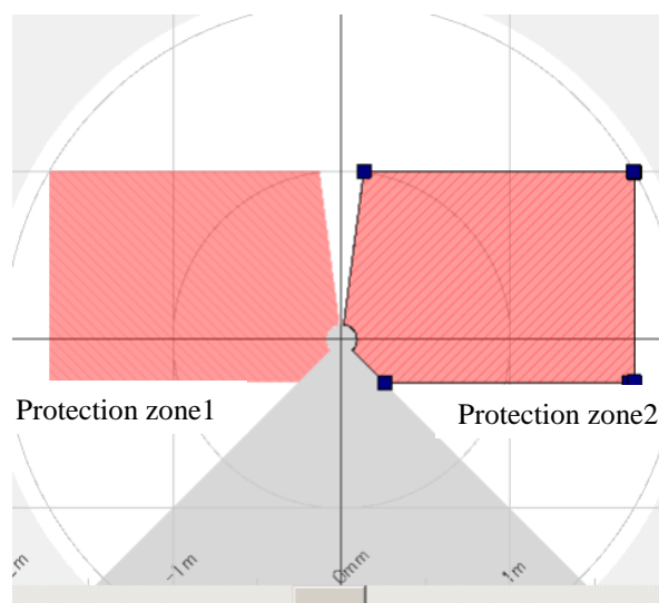
Figure4-3 Example of Dual protection zone configuration
