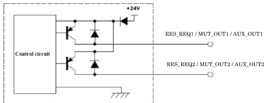
Figure 6-2 Output circuit
