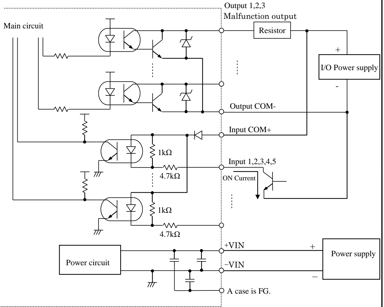
Figure 5: Connection example of inputs, outputs and power supply
